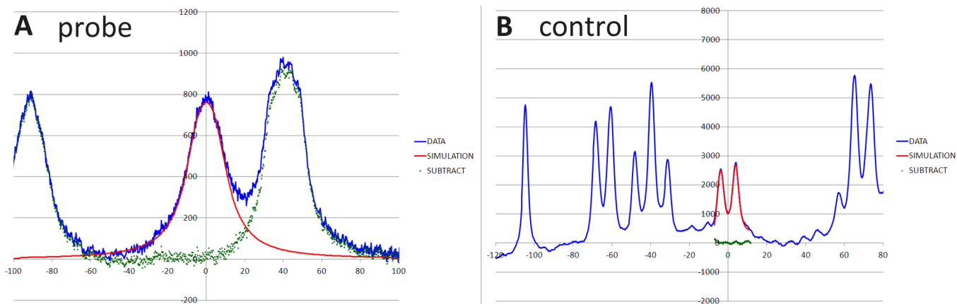
Figure 2. A line width comparison for two Trp He3 resonances of WW st29 at 325 K. The left panel, A, illustrates the signal from the edge-Trp of the turn-flanking Trp/Trp pair which is surrounded by exchange-broadened H_\alpha signals. The right panel, B, illustrates a Trp He3 which displays no structuring shift and thus no exchange broadening. The scale in both panels is in Hertz about the peak center. The red lines (both panels) show simulated Trp He3 7.8 Hz doublets (including broadening associated with two smaller coupling constants, 0.8 and 1.2 Hz) with different amounts of additional line broadening added. The additional line broadening required to fit the exchange broadened peak (difference between left and right panels) provides \Delta^{ex} for the calculation of folding dynamics. 18,21
