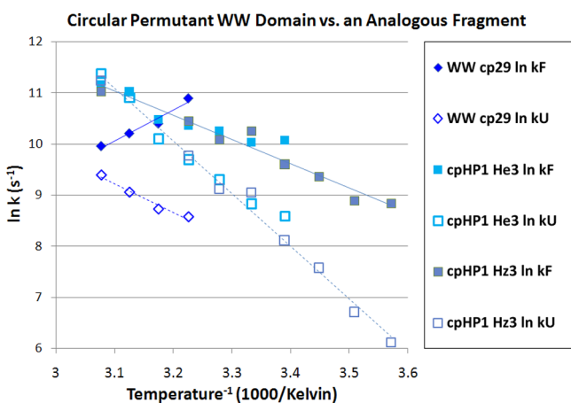
Figure 8. Inverse log plots for folding and unfolding rates of WW cp29 and hairpin fragment cpHP1. In the case of the hairpin, rate data from two ring-current shifted sites (W17 He3 and Hz3) are shown: the lines represent a single linear fit to all of the data.
