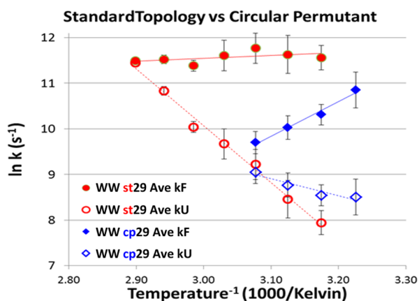
Figure 7. Upper panel: locations of the probes in the WW domain fold (illustrated as gold spheres on the NMR structure of the circular permutant). Lower panel: Arrhenius plots for folding and unfolding rates of the standard-topology WW domain (st29) and its circular permutant (cp29). The points are data averaged over all available probes at each temperature. The probe identities and individual \ln k values appear in the SI (Figure S8).
